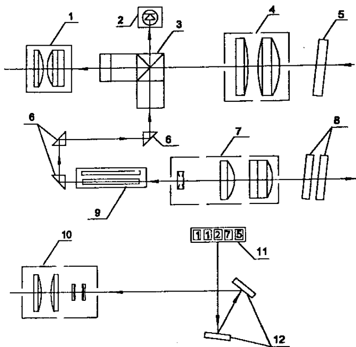
Fig.4. Optical configuration of rangefinder :
